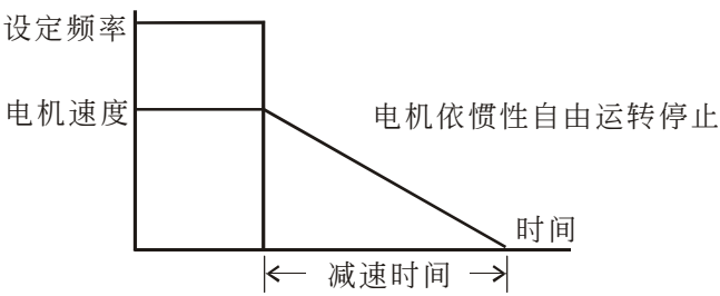
ON OFF 图二：自由运转
